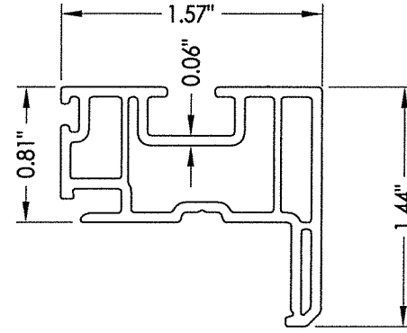
5 TOP RAIL
