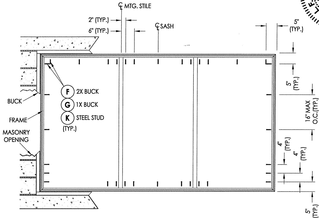
FRAME ANCHORING
