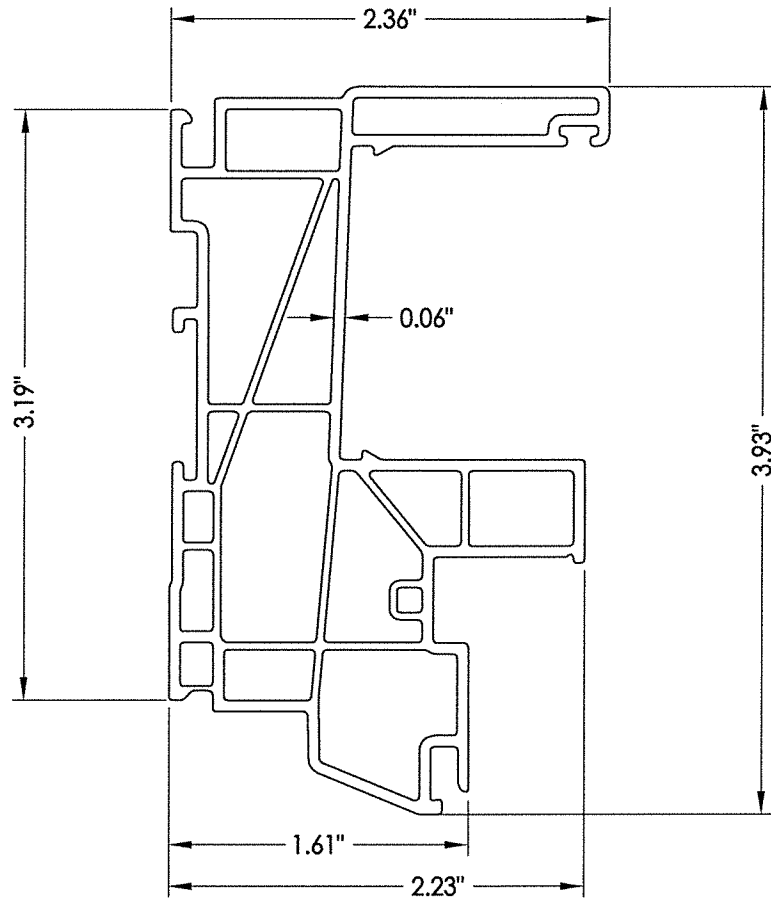
1 FRAME
